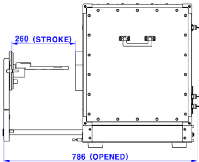
Side View(Opened)
