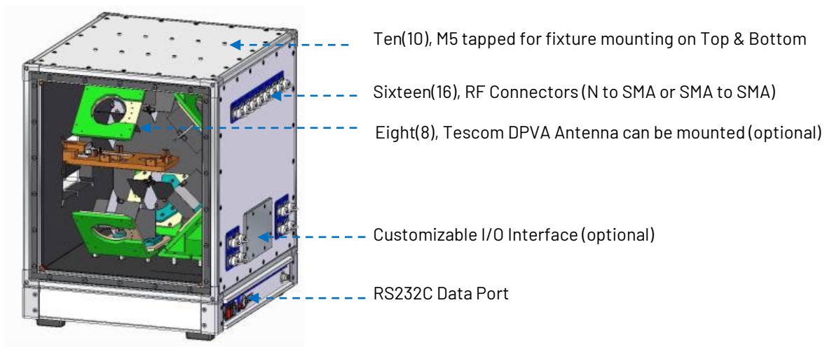
Basic Features(Cross-Section)
