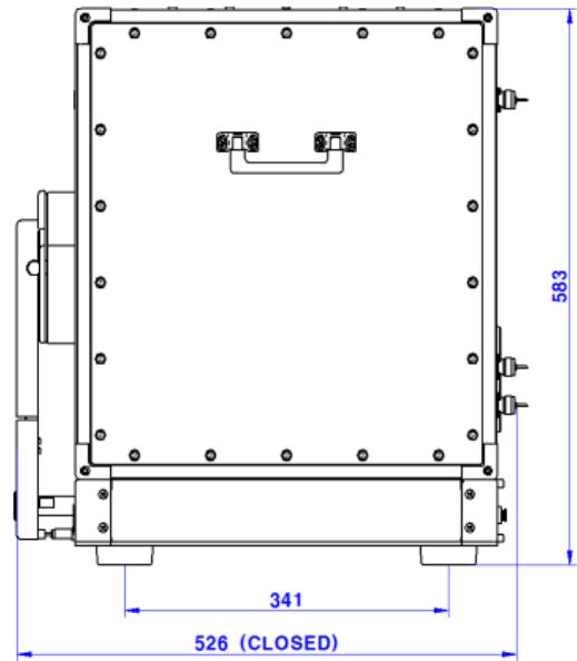
Side View(Closed)
