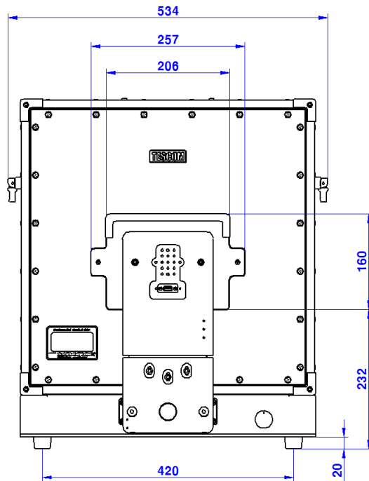
Front View(Closed)
