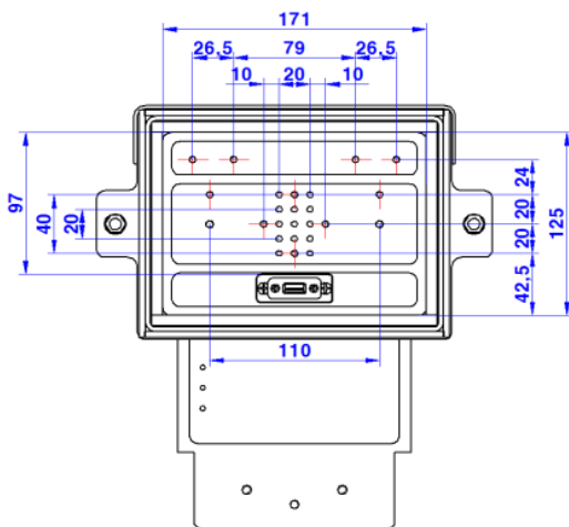
Door View
