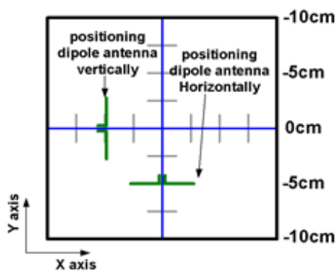
Positioning Dipole Antenna
