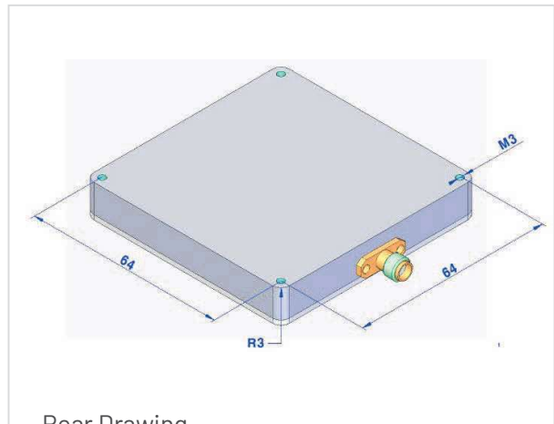
Rear Drawing
