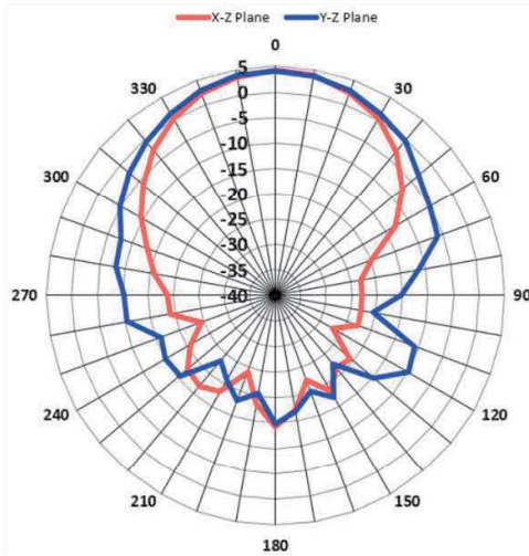
5.0GHz
