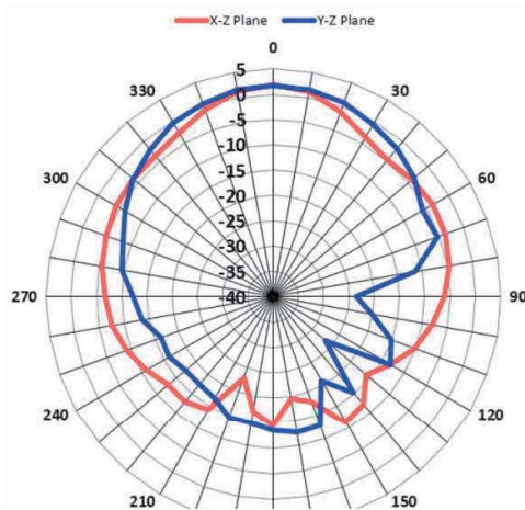
6.0GHz
