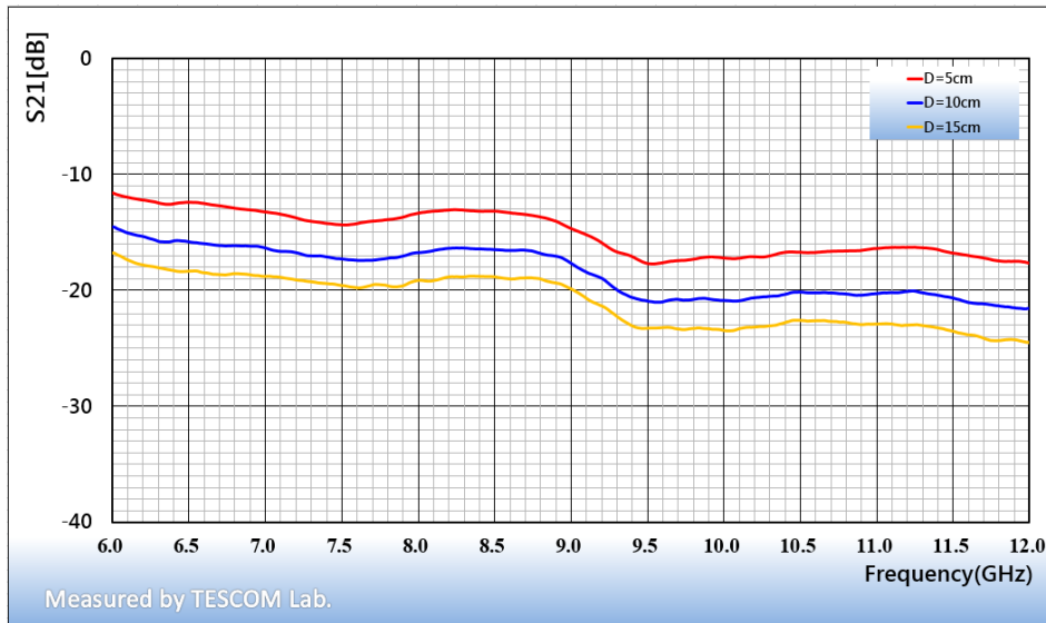
Graph2. TC-93177A Path-Loss(Horizontal)
