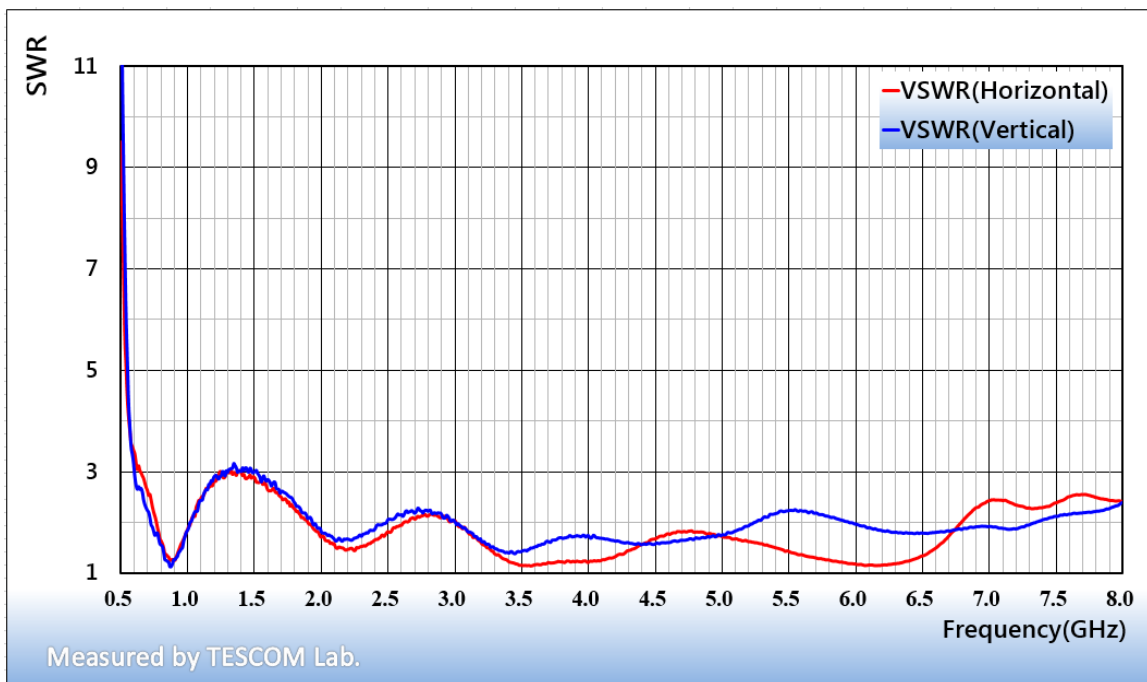
Graph 1. TC-93083A VSWR
