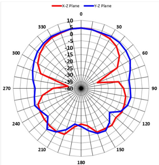
4.0GHz_Vertical
