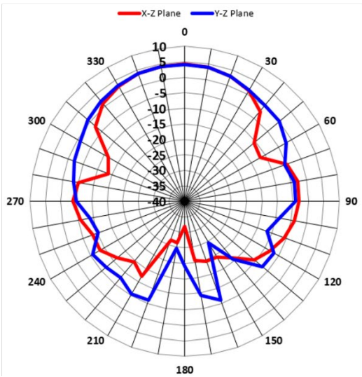
6.0GHz_Vertical
