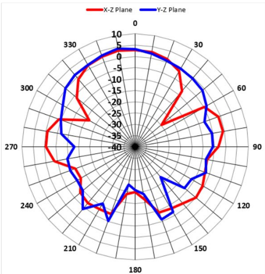
7.0GHz_Vertical
