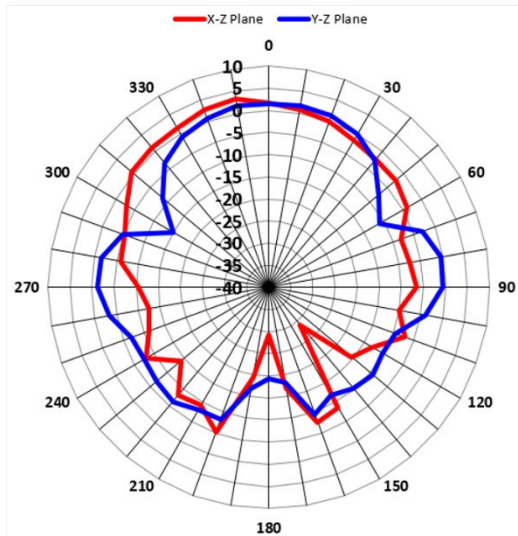
7.0GHz_Horizontal
