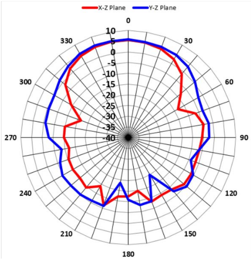
5.5GHz_Vertical
