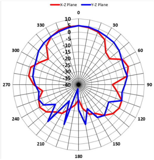
7.5GHz_Vertical
