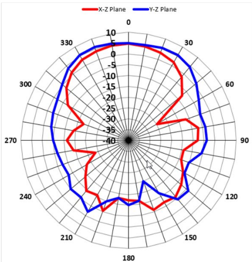
5.0GHz_Vertical
