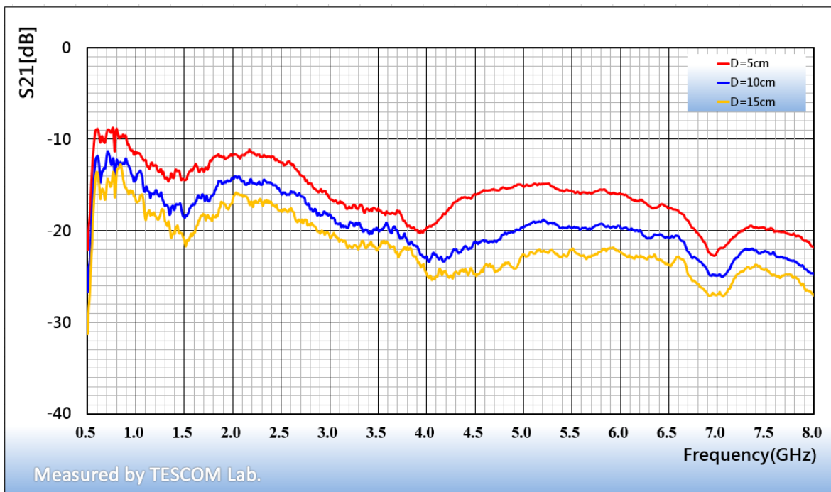
Graph 4. TC-93083A Path-Loss (Vertical)
