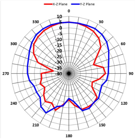
4.5GHz_Vertical
