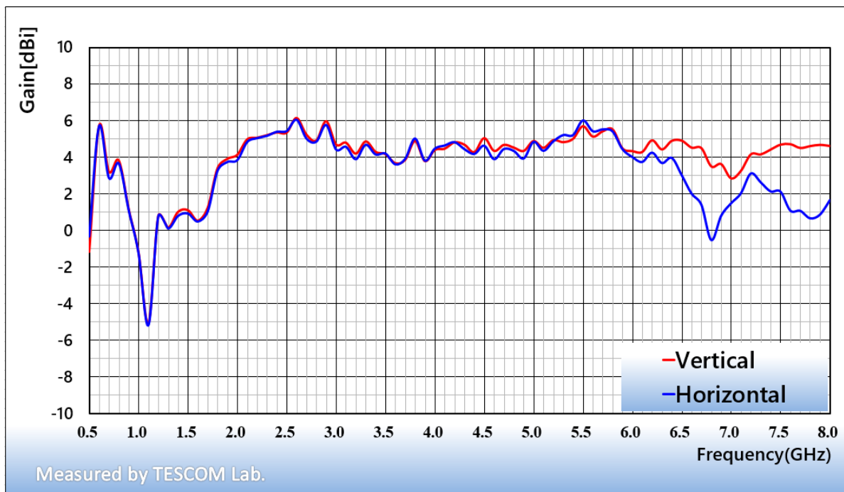
Graph 2. TC-93083A Gain
