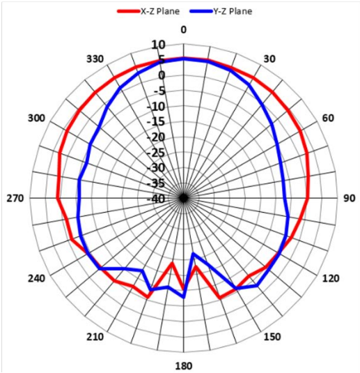
2.4GHz_Vertical
