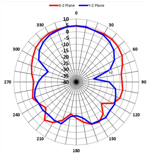
4.0GHz_Horizontal
