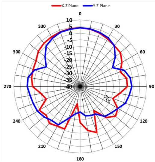
6.0GHz_Horizontal
