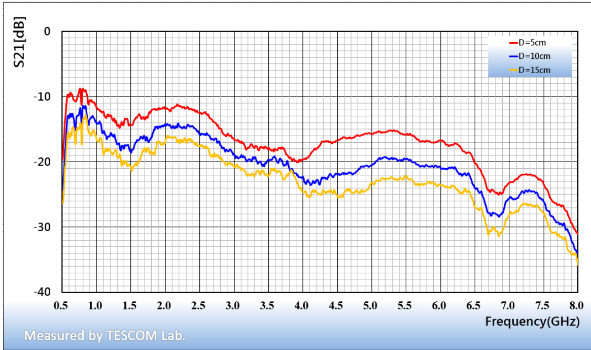
Graph 3. TC-93083A Path-Loss (Horizontal)
