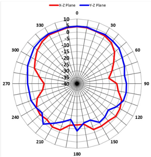
3.5GHz_Vertical
