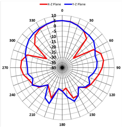
6.5GHz_Vertical
