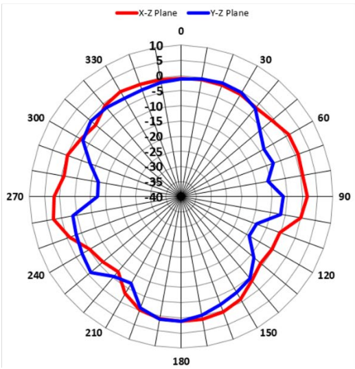
0.6GHz_Vertical
