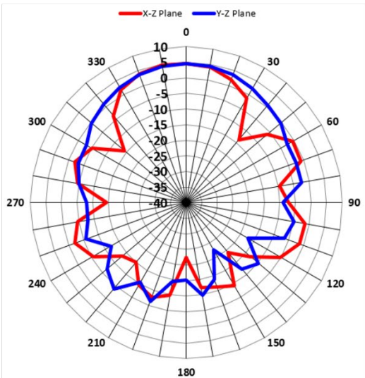
8.0GHz_Vertical
