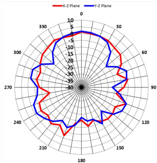
8.0GHz_Horizontal
