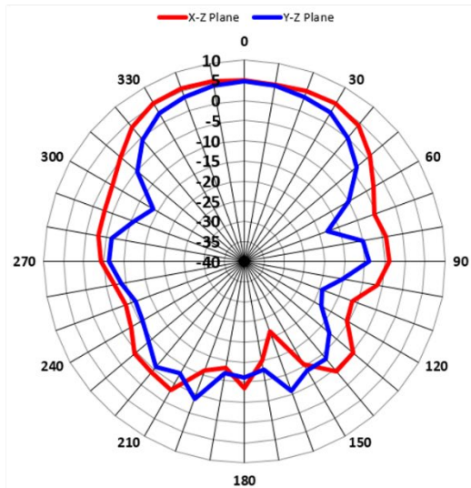
5.0GHz_Horizontal
