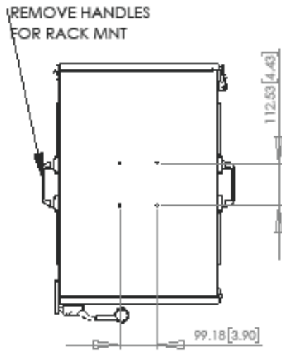
4 X M4 INT ROOF MOUNT POINTS
